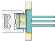
Component Housing
