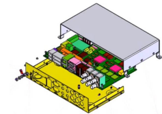
Housing Adaptation
